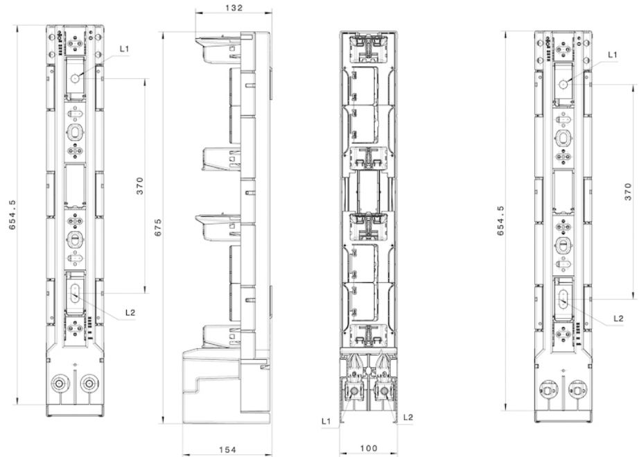
Steel-frame clamp KM2G-F
