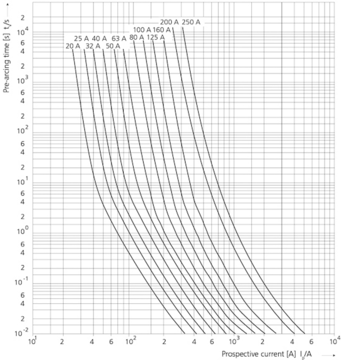
Time-current characteristics
