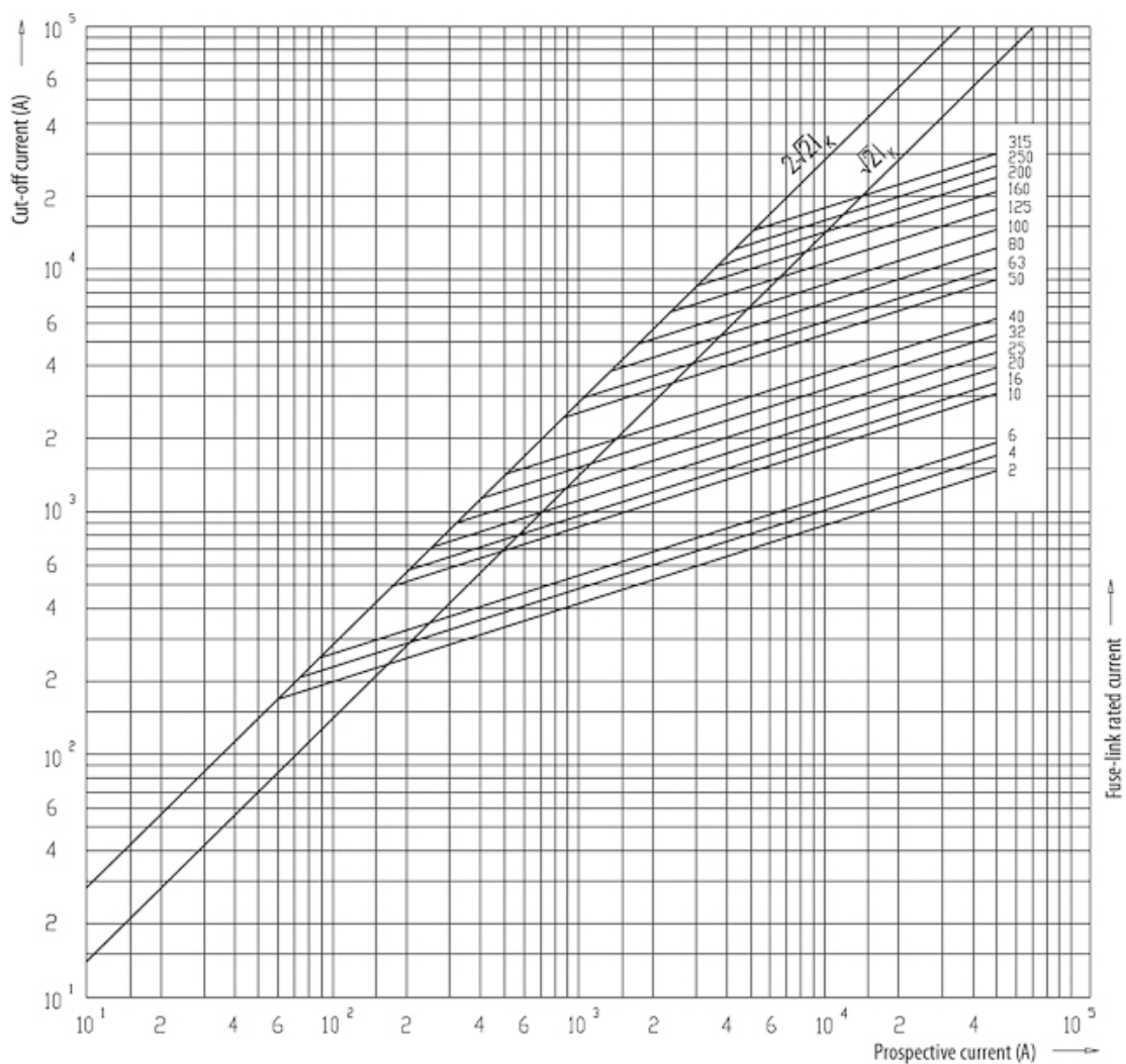
Cut-off current diagram for VV-Thermo fuse links
